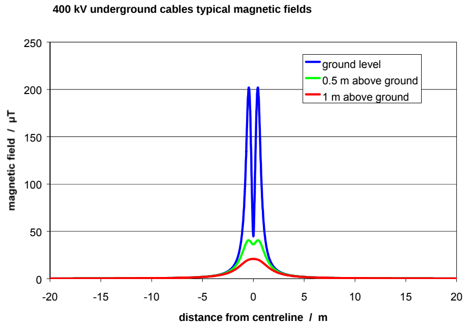
Figure 8 Magnetic fields from underground transmission cable
